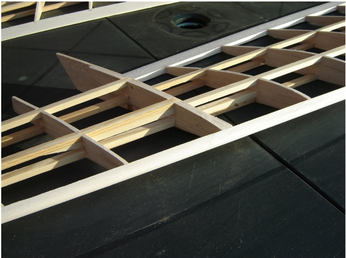
Construction where the wing tip is attached to the main wing section.
